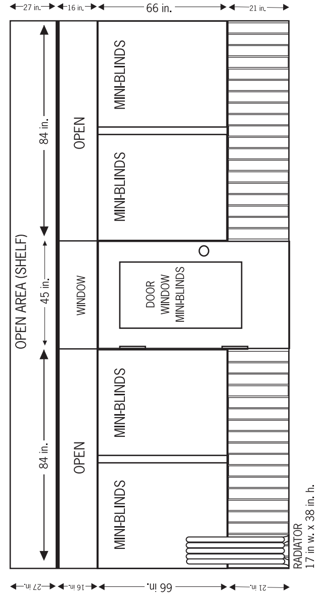
SHOP WINDOWS LAYOUT (VIEW FROM INSIDE GALLERY)
